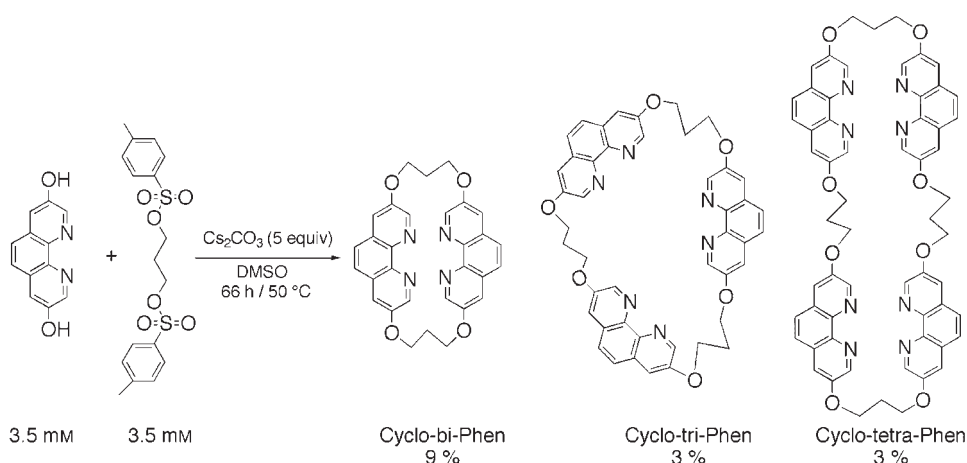
Scheme 1. Synthesis of "Cyclo-Phen".
