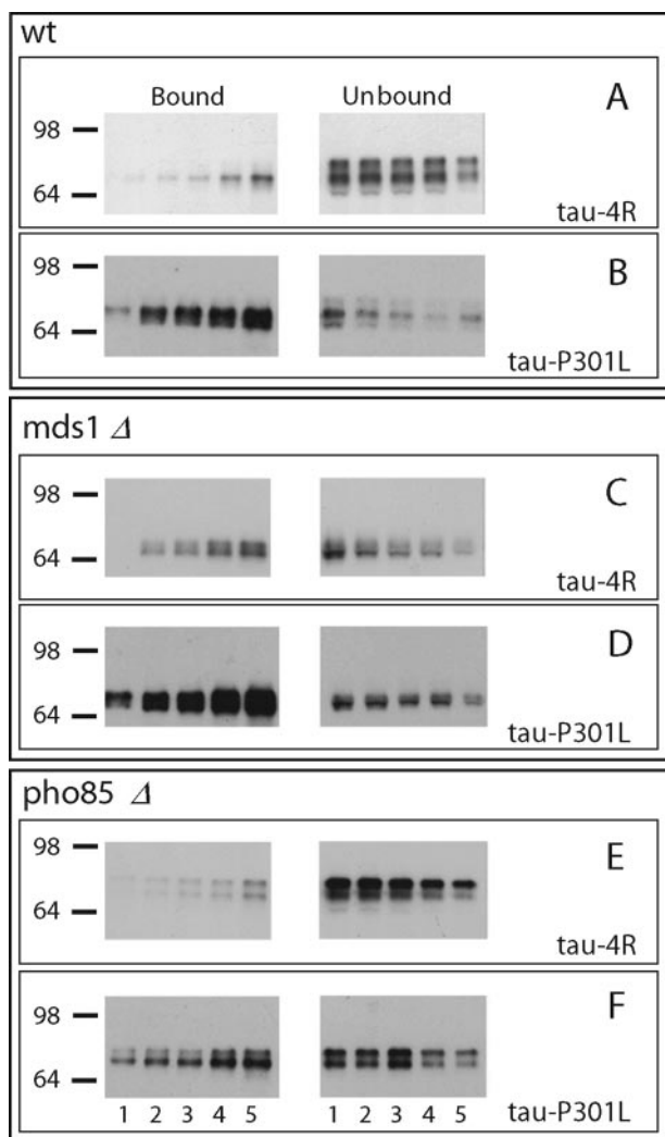
FIGURE 4. In vitro binding of monomeric Tau-4R (A, C, and E) and Tau-P301L (B, D, and F) on Taxol-stabilized MT determined by SDS-PAGE and Western blotting using pan-Tau mAb Tau-5. Bound and unbound fractions of BY4741-Tau (A and B), \Delta mds1 -Tau (C and D), and \Delta pho85 -Tau (E and F) to 0 (lane 1), 0.8 (lane 2), 1.5 (lane 3), 3 (lane 4), and 6 \mu\text{M} MT (lane 5).
