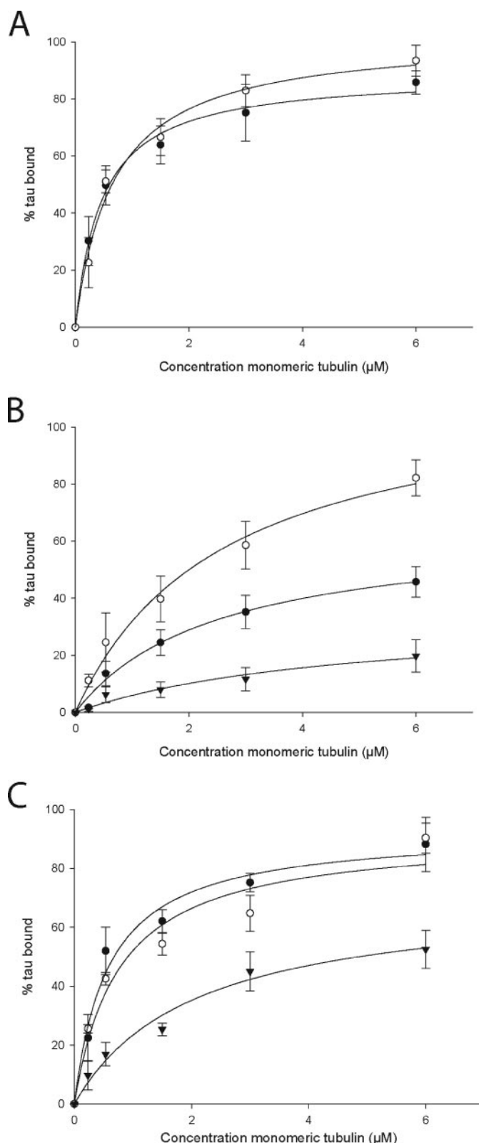
FIGURE 5. Quantification of the in vitro binding of wild type Tau-4R and mutant Tau-P301L to Taxol-stabilized MT. A, relative amount of bound dephosphorylated wild type Tau-4R (black circles) and Tau-P301L (open circles); B, BY4741-Tau-4R (black circles), \Delta mds1 -Tau-4R (open circles), and \Delta pho85 -Tau-4R (black triangles); and C, BY4741-Tau-P301L (black circles), \Delta mds1 -Tau-P301L (open circles), and \Delta pho85 -Tau-P301L (black triangles) were plotted to the concentration of monomeric tubulin to determine Tau binding characteristics (see "Experimental Procedures" and Table 2). All data are mean \pm S.E. of 3 independent experiments.
