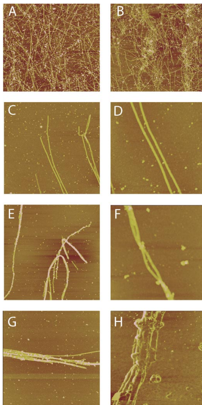
FIGURE 6. Ultrastructural analysis of Taxol-stabilized MT incubated with or without different phosphorylated wild type or mutant Tau forms by AFM. A and B, incubation of 10 \mu\text{m} MT without (A) and with (B) pig MAPs. Field widths are 20 \mu\text{m} . C and D, incubation of 1.5 \mu\text{m} MT with BY4741-Tau-4R displays no apparent changes in morphology of MT. Most MT are 8 nm in height and separately dispersed on the silicon surface, only coincidental MT crossing was observed and a complete absence of clustering on the MT surface. Field widths are 5 and 1.5 \mu\text{m} for C and D, respectively. E–H, incubation of 1.5 \mu\text{m} MT with BY4741-Tau-P301L display a drastic change in MT morphology causing clusters on the MT surface and causes MT to stick together and bend abnormally (E and F). At the end of these irregular structures, individual MT can be observed covered with Tau clusters (G) and high-resolution phase images clearly demonstrate a severely disturbed surface of MT with coagulated Tau-P301L (H). Field widths are 7, 1.5, 5, and 700 nm, respectively.
