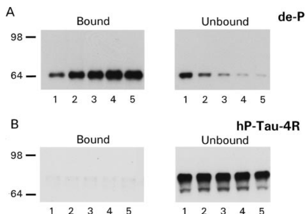
FIGURE 3. In vitro binding of isolated hP-Tau/MC1 monomers on Taxol-stabilized MT determined by SDS-PAGE and Western blotting using pan-Tau mAb Tau-5. A and B, bound and unbound fractions of dephosphorylated Tau-4R (A) and hP-Tau-4R (B) to 0 (lane 1), 0.8 (lane 2), 1.5 (lane 3), 3 (lane 4), and 6 \mu M MT (lane 5).
