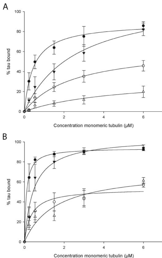
FIGURE 2. Quantification of the in vitro binding of isolated Tau-4R monomers (A) or dimers (B) to Taxol-stabilized MT. Relative amount of bound dephosphorylated Tau (black circles), BY4741-Tau (open circles), \Delta\text{mds1} -Tau (black triangles), and \Delta\text{pho85} -Tau (open triangles) were plotted to the concentration of monomeric tubulin to determine Tau binding characteristics (see "Experimental Procedures" and Table 2). All data are mean \pm S.E. of 3 independent experiments.
